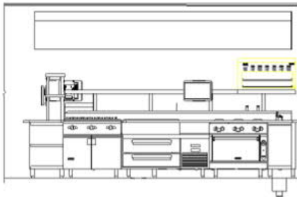
13 EXPO KITCHEN - CHEF'S COUNTER, RIGHT 1/2" = 1'-0"
