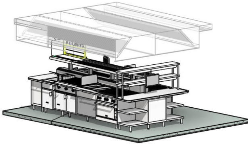
④ EXPO KITCHEN - ISLAND, 3D NTS
