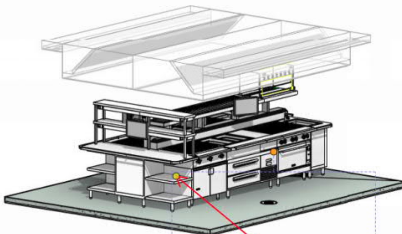
5 EXPO KITCHEN - ISLAND, 3D NTS
